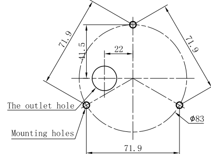
Mounting holes
