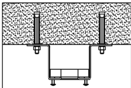
1-CEILING-MOUNT BRACKET
