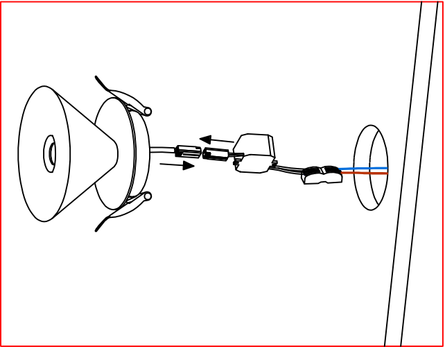
3. Connect de LED cable to the driver cable.
