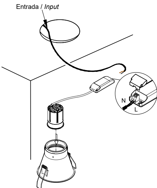
FIG-3a MÓDULO LED / LED MODULE
