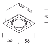
egypt 5 CUT OUT 50x50 mm MIN. HEIGHT 55 mm
