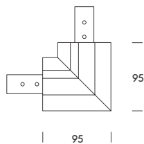
2 5 Right L joint | Left L joint
