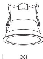
libertad 6 CUT OUT Ø68 mm MIN. HEIGHT 90 mm
