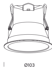
libertad 9 CUT OUT Ø90 mm MIN. HEIGHT 100 mm
