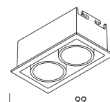
egypt 10 CUT OUT 50x90 mm MIN. HEIGHT 55 mm
